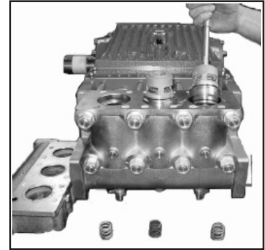
3) Take out pressure springs (57A). Pull out assembled valves (51 & 52) with valve
